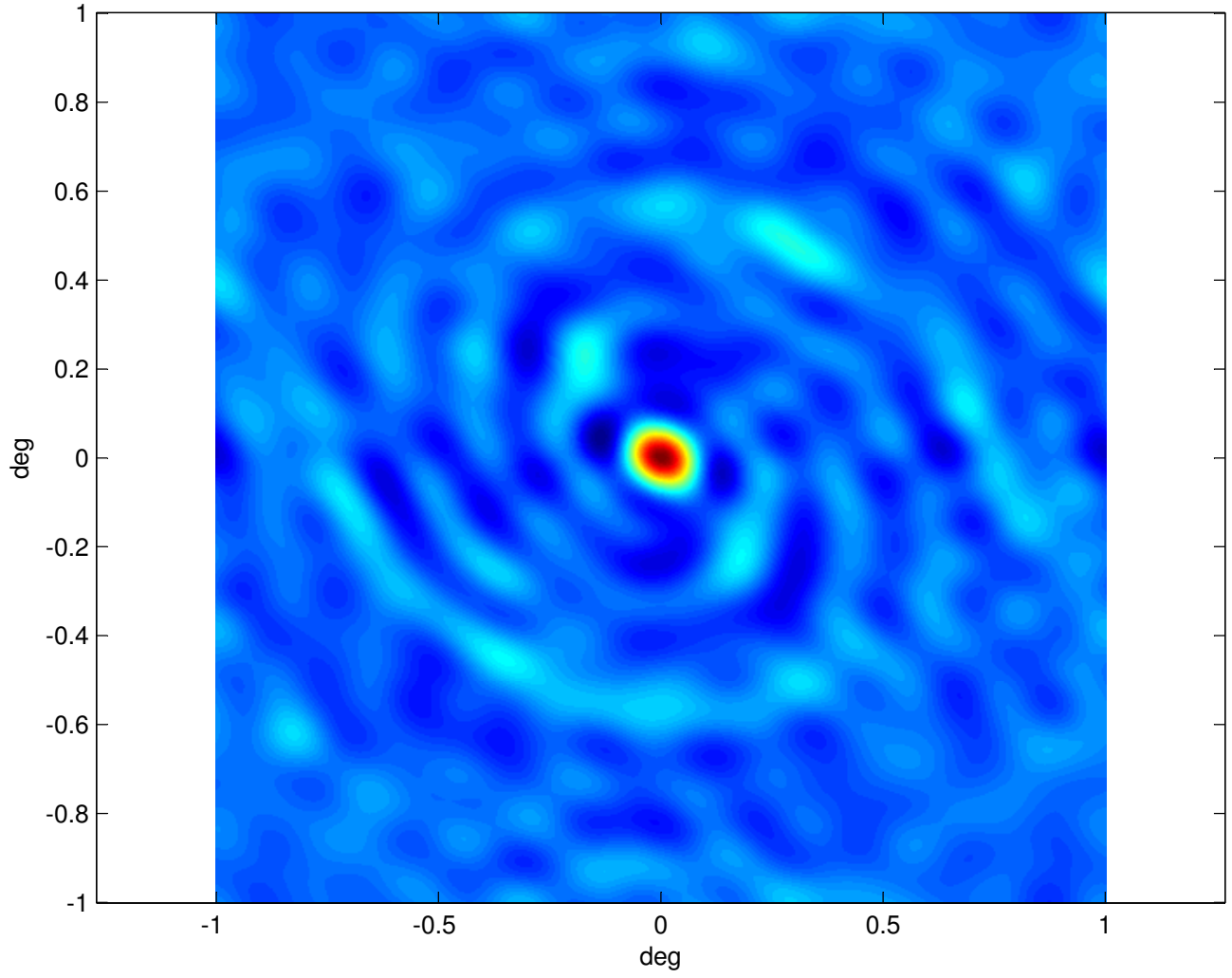
Cassiopeia A (cell averaging)
